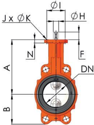
Dimensions DN 32-600
