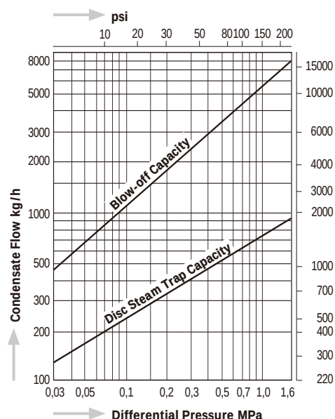
Capacity Chart SV-N
