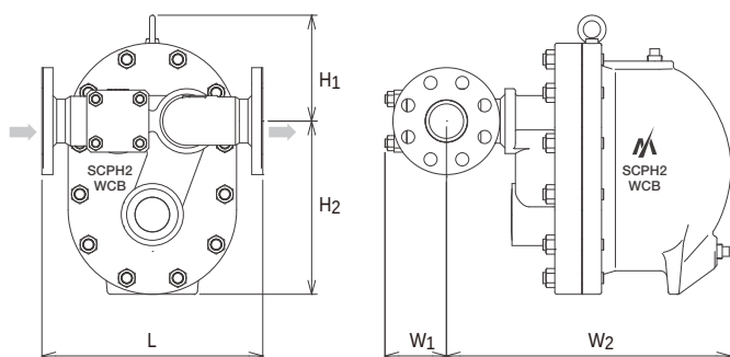
Dimensions GH60
