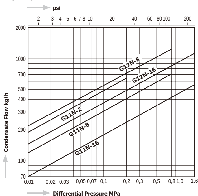
Capacity Chart G11N, G12N
