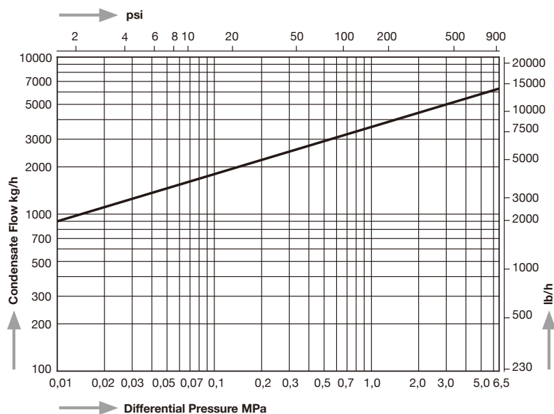
Capacity Chart GWH70
