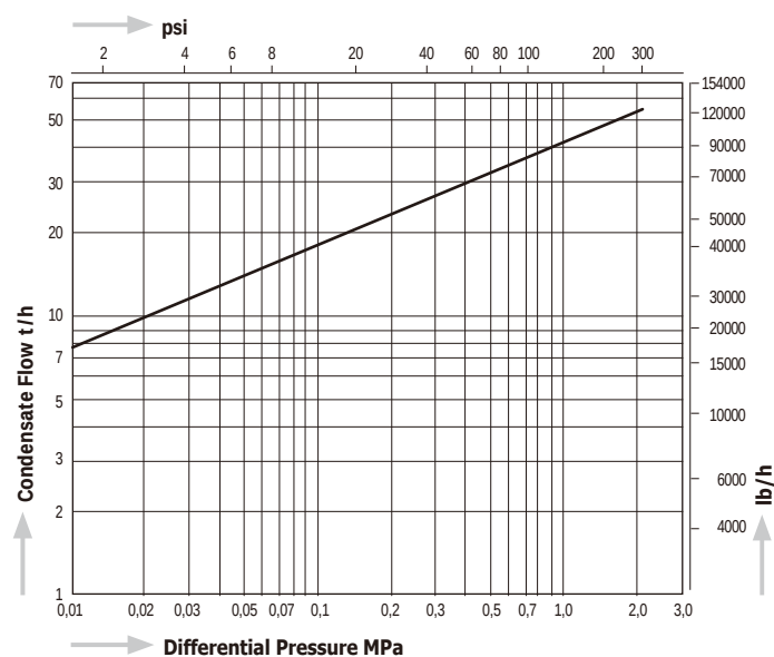
Capacity Chart GH70
