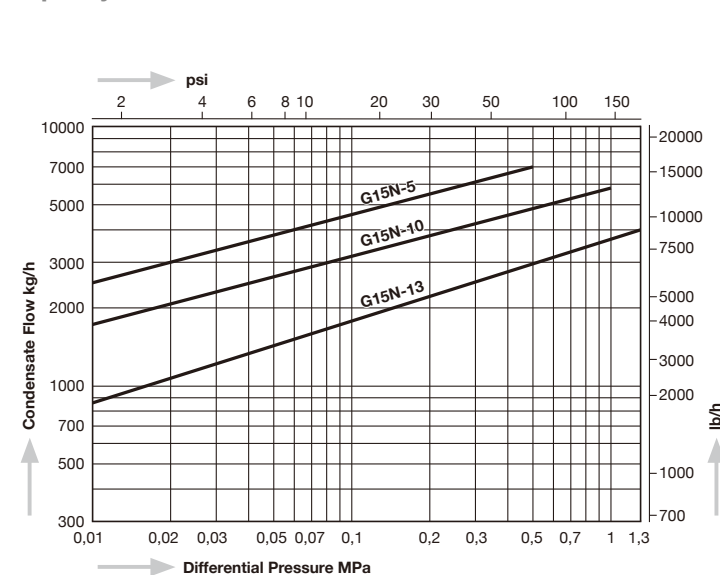
Capacity Chart G15N
